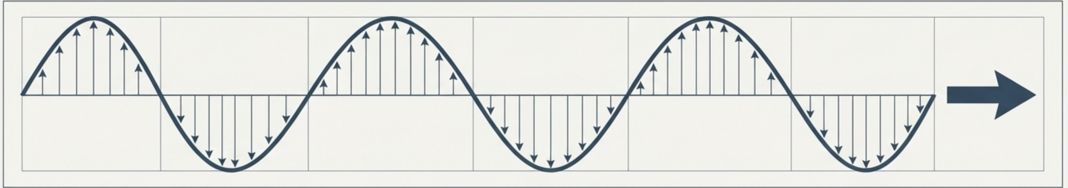
Transverse Wave: Scatters Energy, Contributes Heat
