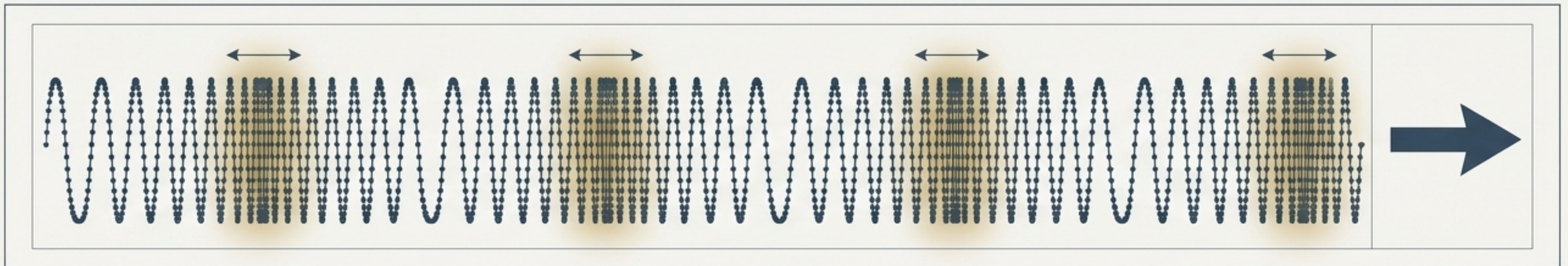
Longitudinal Wave: Focuses Energy, Enables Implosion
