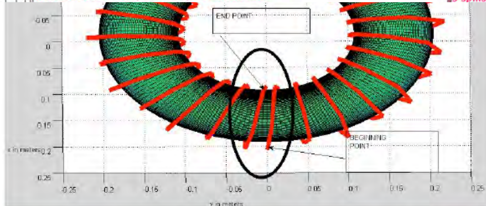
Figure 1. A toroid wrapped 26.5 times. We have found that symmetrical wrappings produce no thrust, whereas wrappings such as this produce thrust at harmonics of a computed frequency.
